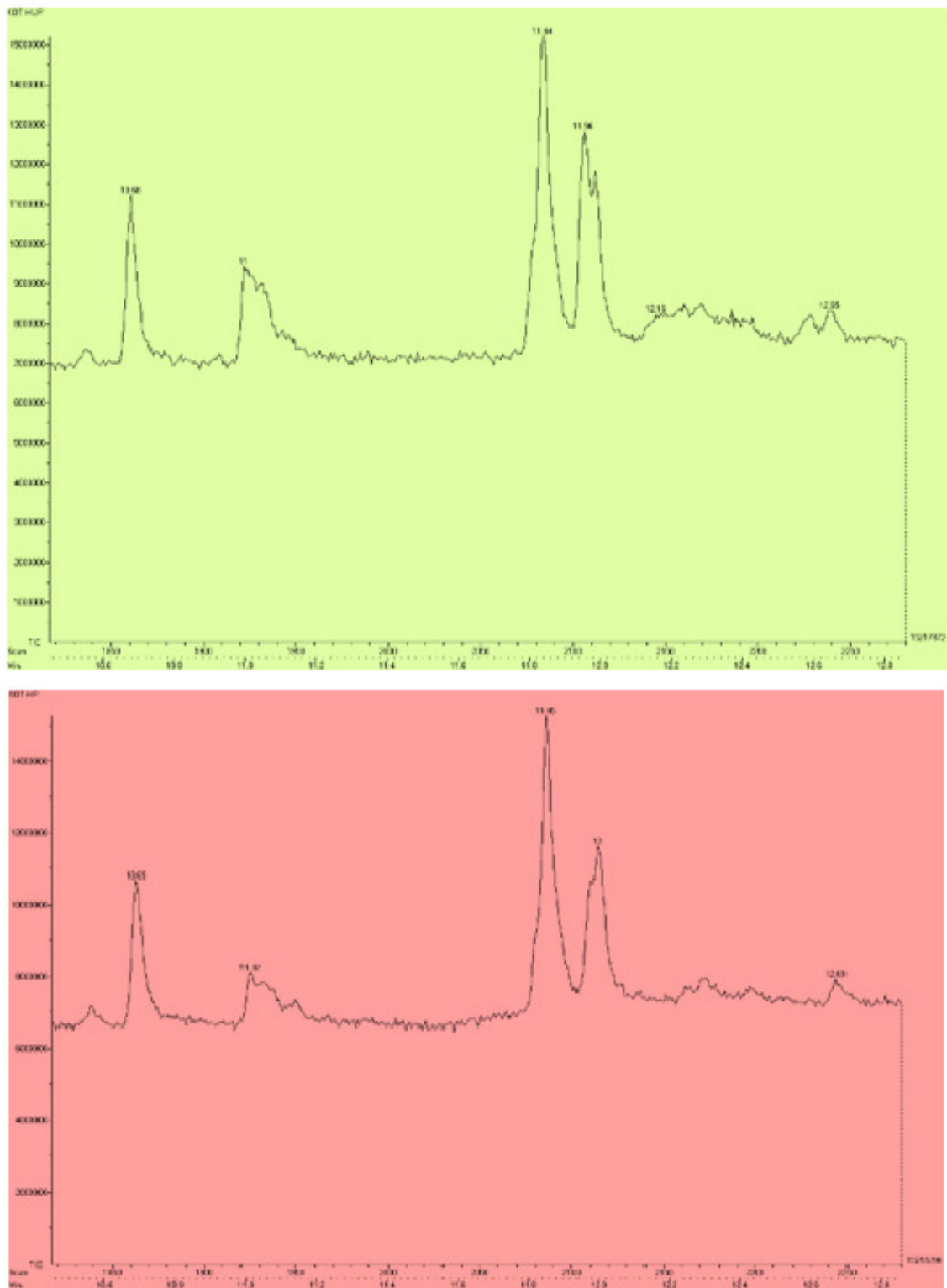
Fig. 1. GC-MS chromatogram of the ethanol extract of H. verticillata collected from unpolluted and polluted water sources
