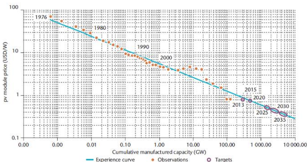
Fig. 4. Photovoltaic modules old prices and 2035 projection [21]
