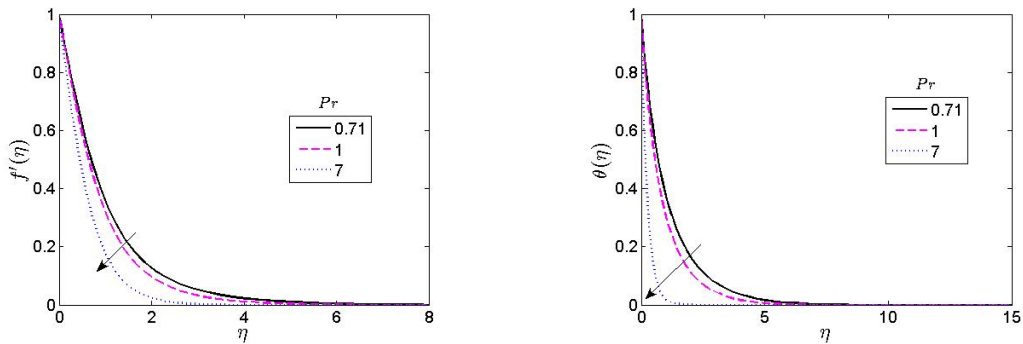
Fig. 4. Velocity and Temperature profiles for different values of Prandtl number Pr
