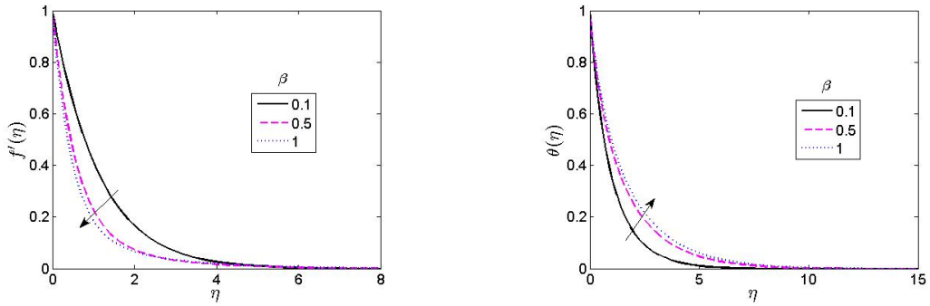
Fig. 5. Velocity and Temperature profiles for different values of casson parameter \beta
