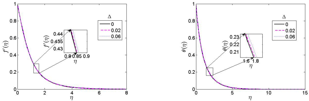
Fig. 7. Velocity and Temperature profiles for different values of heat generation parameter \Delta
