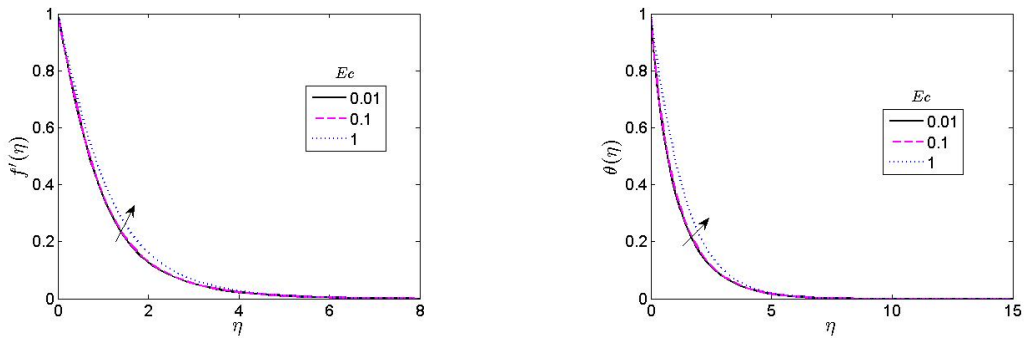
Fig. 6. Velocity and Temperature profiles for different values of Eckert number Ec
