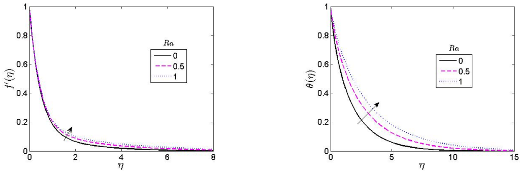
Fig. 8. Velocity and Temperature profiles for different values of thermal radiation parameter Ra
