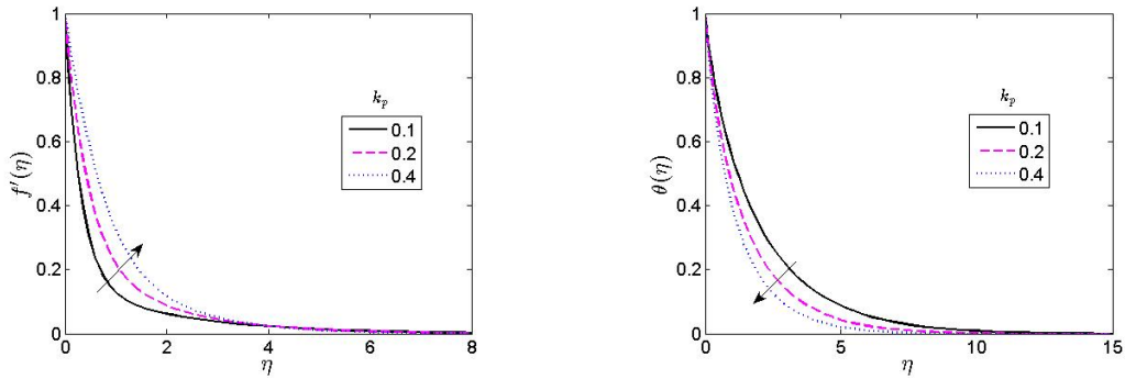
Fig. 3. Velocity and Temperature profiles for different values of permeability parameter k_p
