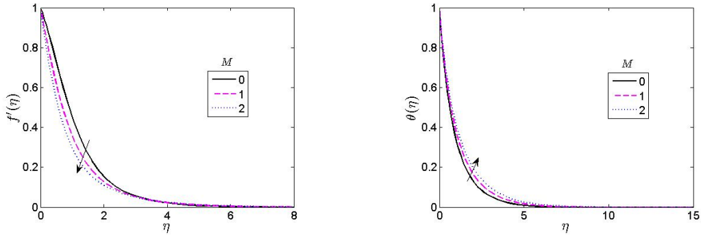
Fig. 2. Velocity and Temperature profiles for different values of Magnetic parameter M
