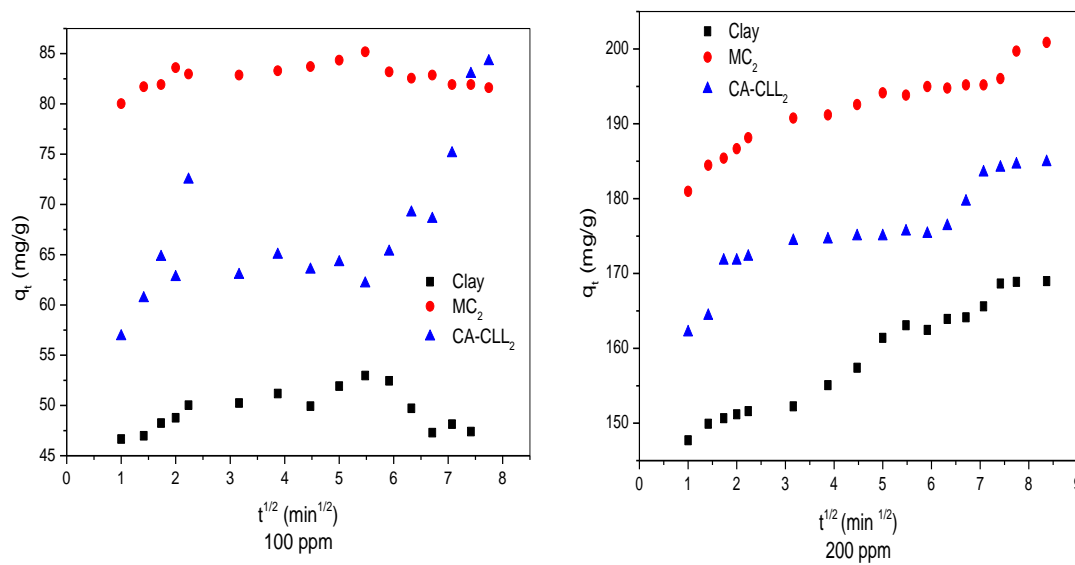
Fig.6. Intraparticle diffusion for the adsorption of Congo red on adsorbent materials.
