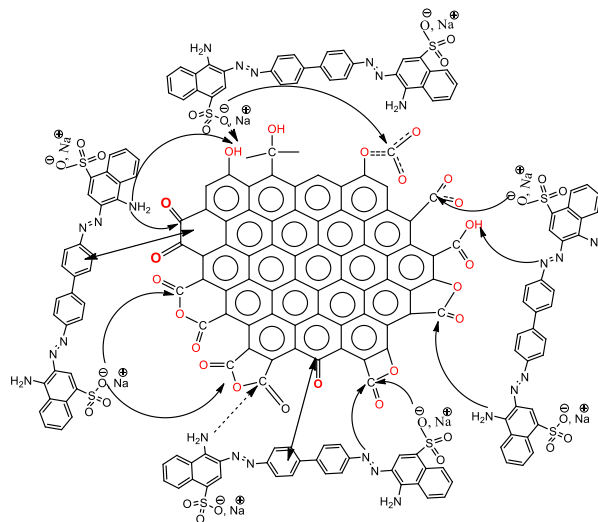
Fig. 12. Adsorption mechanism of red Congo on adsorbent materials [16]
