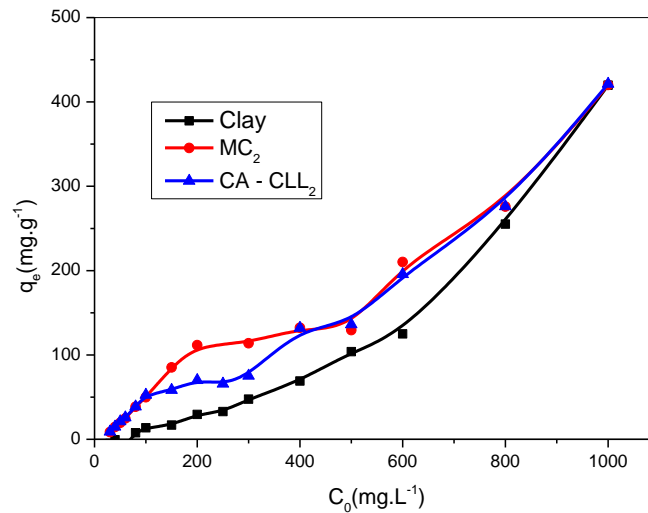
Fig.3. Effect of initial concentration on the adsorption capacity of red Congo on the three adsorbents
