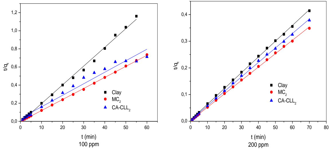
Fig. 5. Linearized forms of the pseudo-second-order model for the adsorption of Congo red on adsorbent materials
