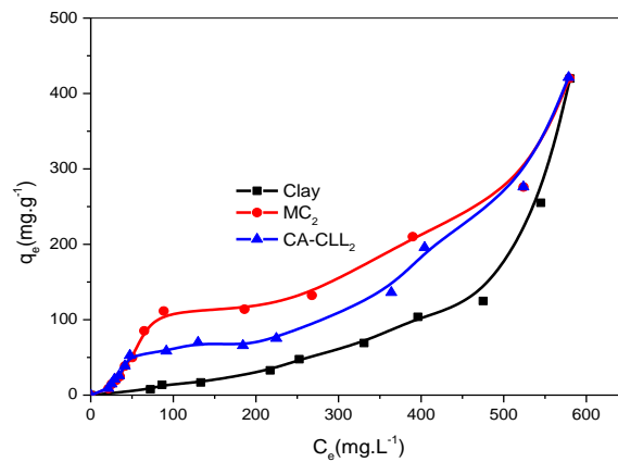
Fig. 8. Isotherms' adsorption of red Congo on adsorbent materials
