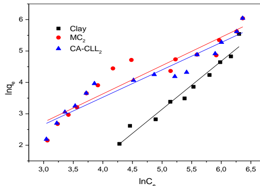
Fig. 10. Forms linearized of the model Freundlich for red Congo adsorption on the three adsorbent materials
