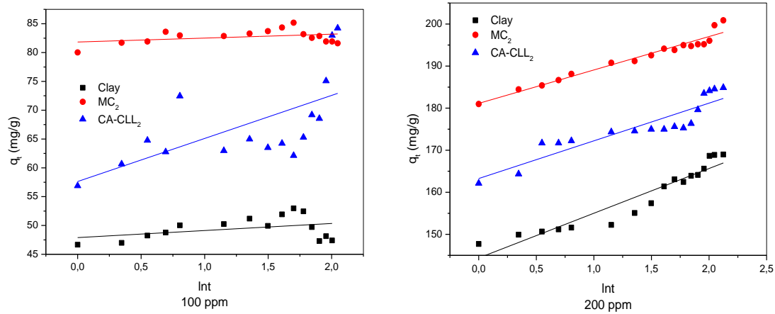
Fig. 7. Linearized forms of the Elovich model for the adsorption of Congo red on adsorbent materials
