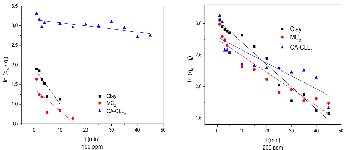
Fig. 4. Linearized forms of the pseudo-first-order model for the adsorption of Congo red on adsorbent materials
