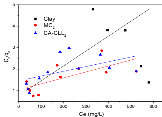
Fig. 9. Forms linearized of the model Langmuir for red Congo adsorption on the three adsorbent materials
