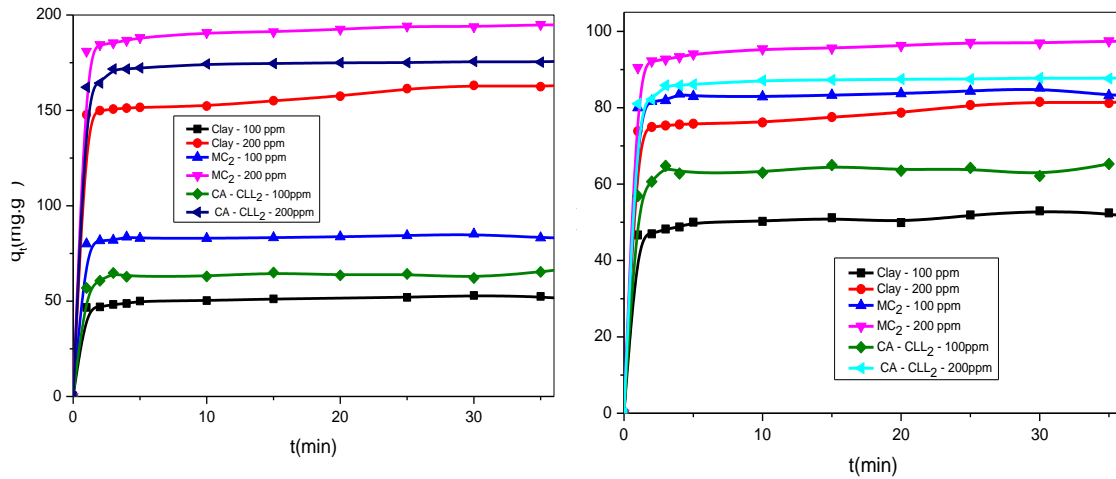
Fig. 2. Influence of time and initial concentration on the amount and rate of adsorption of Congo red by three adsorbents
