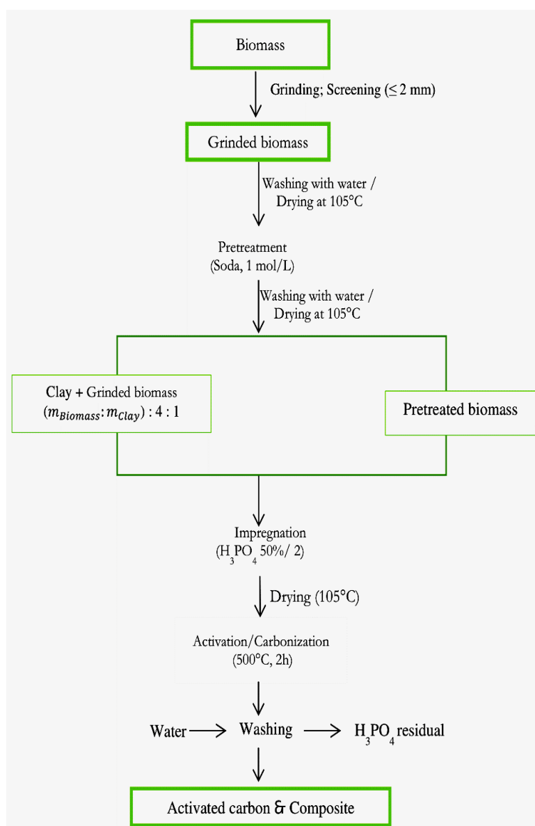
Fig. 1. Different steps in the elaboration the adsorbants
