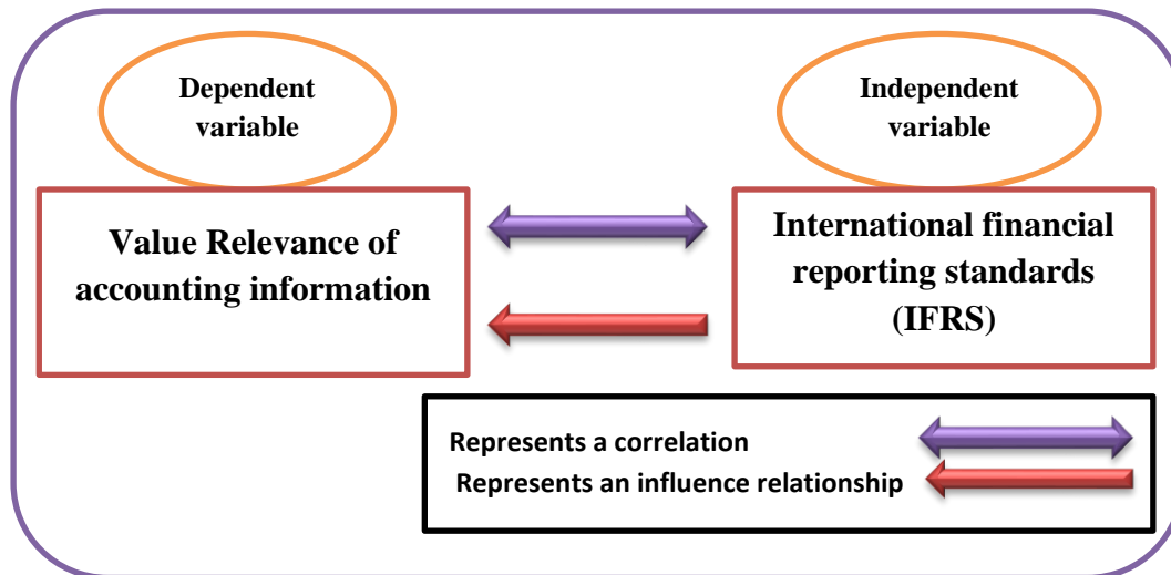
Fig. 1. Research model
