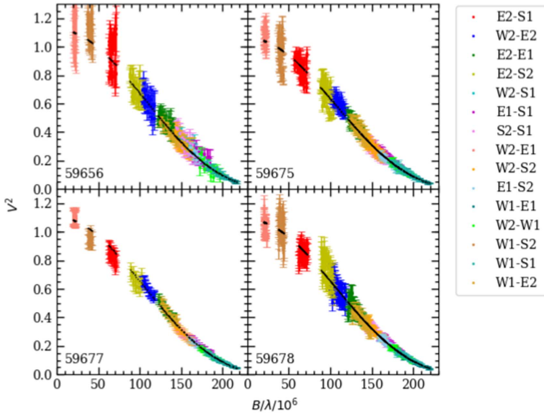
Figure 8. Fits to the interferometric data for the giant 31 Com. The color points show observations with different baselines in the CHARA array, and the black points show the best model fits. Labels give the Julian date of observation–2400000.
