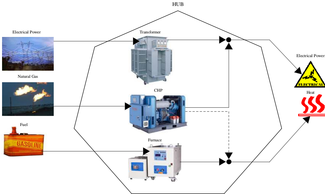
Fig. 1. An integrated energy system (HUB)
