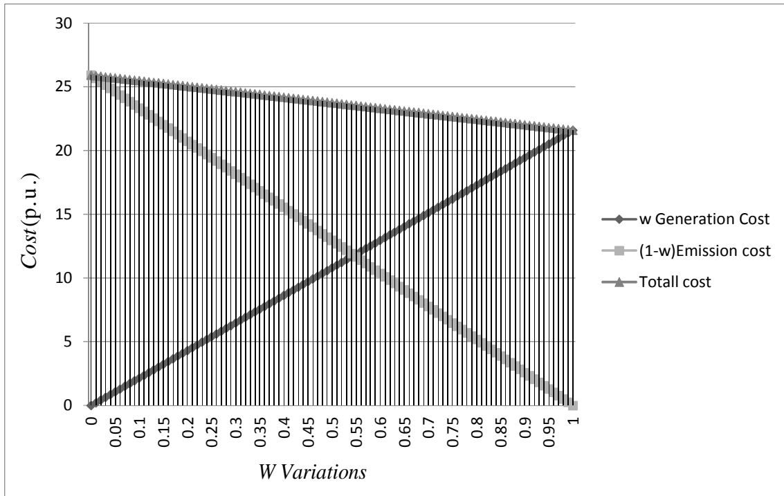
Fig. 4. The W variations effects on the generation, the emission and total cost of the objective function in during 24 hour period
