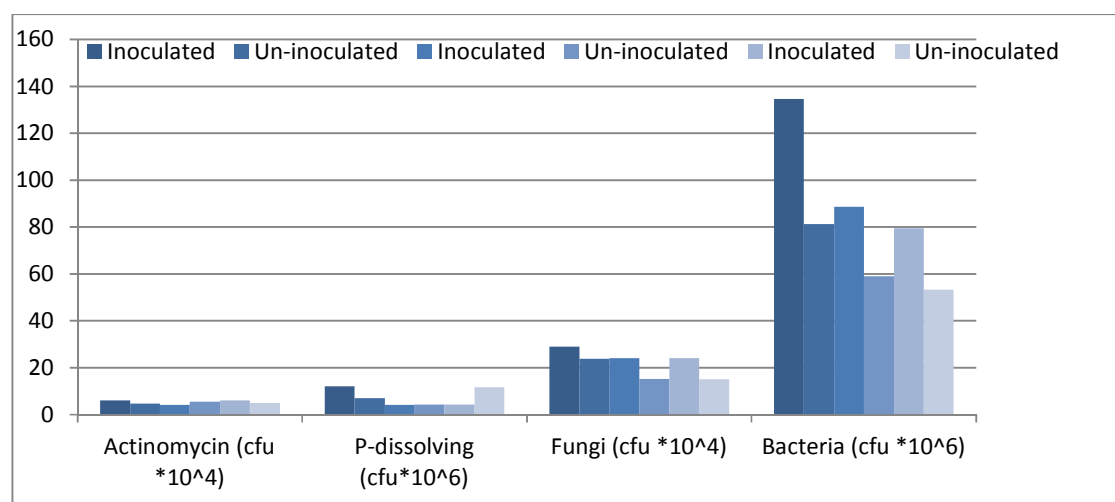
Fig. 3. Showed effect of inoculation and phosphorus fertilization on microbial count of faba bean rhizosphere root at 70 days in pots experiment at salinity level 8.7 dSm -1
