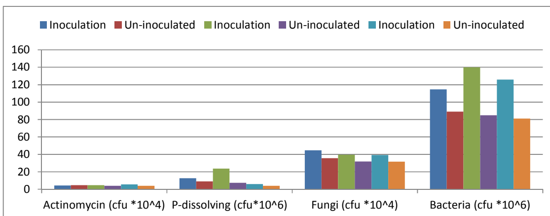
Fig. 2. Showed effect of inoculation and phosphorus fertilization on microbial count of faba bean rhizosphere root at 70 days in pots experiment at salinity level 6.9 dSm -1
