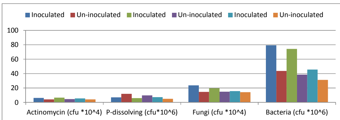
Fig. 1. Showed effect of inoculation and phosphorus fertilization on microbial count of faba bean rhizosphere root at 70 days in pots experiment at salinity level 14.8 dSm -1
