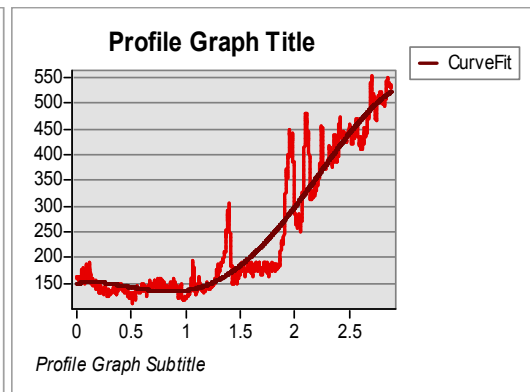
Fig. 5. Cross profile of Indrawati basin
