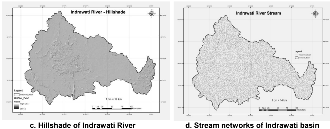
Fig. 3. Basin characteristic map of Indrawati River
