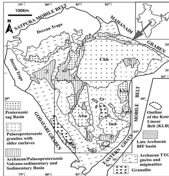
Geological map of the Bastar Craton. Inset in the upper part shows the location of the Bastar and other cratons in India, modified after Ramachandra et al. (2001); (1) Chilpi Belt, (2) Sausar Belt, (3) Amgaon Belt, (4) Kotri Linear Belt, (5) Bengal Belt, (6) Sukma Belt, (7) Sonakhan Belt, Chh = Chhattisgarh Basin, Kha = Kharar Basin, Amp = Amphani Basin, Ind = Indravati Basin, Abu= Abujhmar Basin, Suk = Sukma Basin, Pak = Pakhal Basin. Figure 3. SRTM-DEM image of southern Bastar Craton (studied area).
