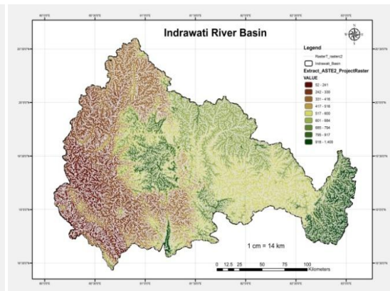
b. River basin of Indrawati
