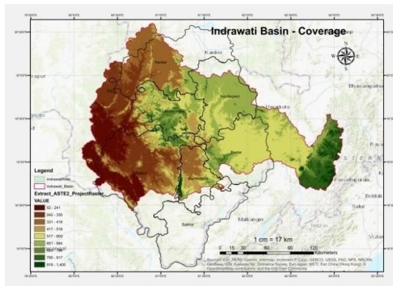
a. Basin coverage of Indrawati River
