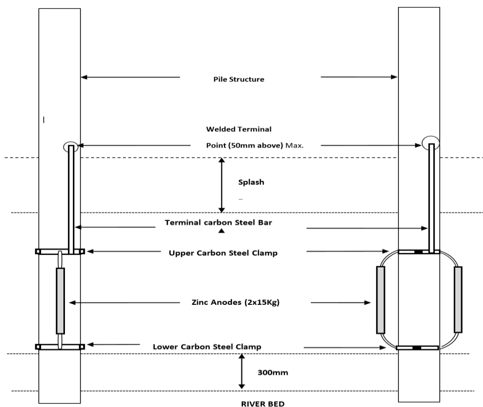
Fig. 5. Layout/configuration of anodes on steel casing piles for the 60 m reinforced concrete bridge
