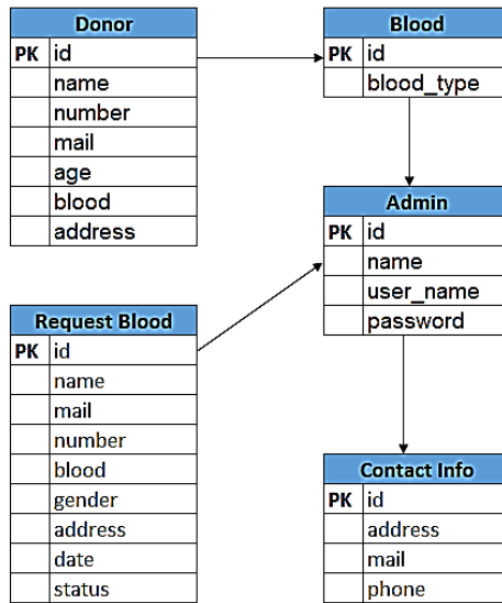
Fig. 5. Entity Relationship Diagram
