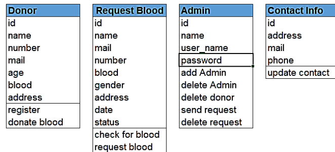
Fig. 6. Object Models of Entities
