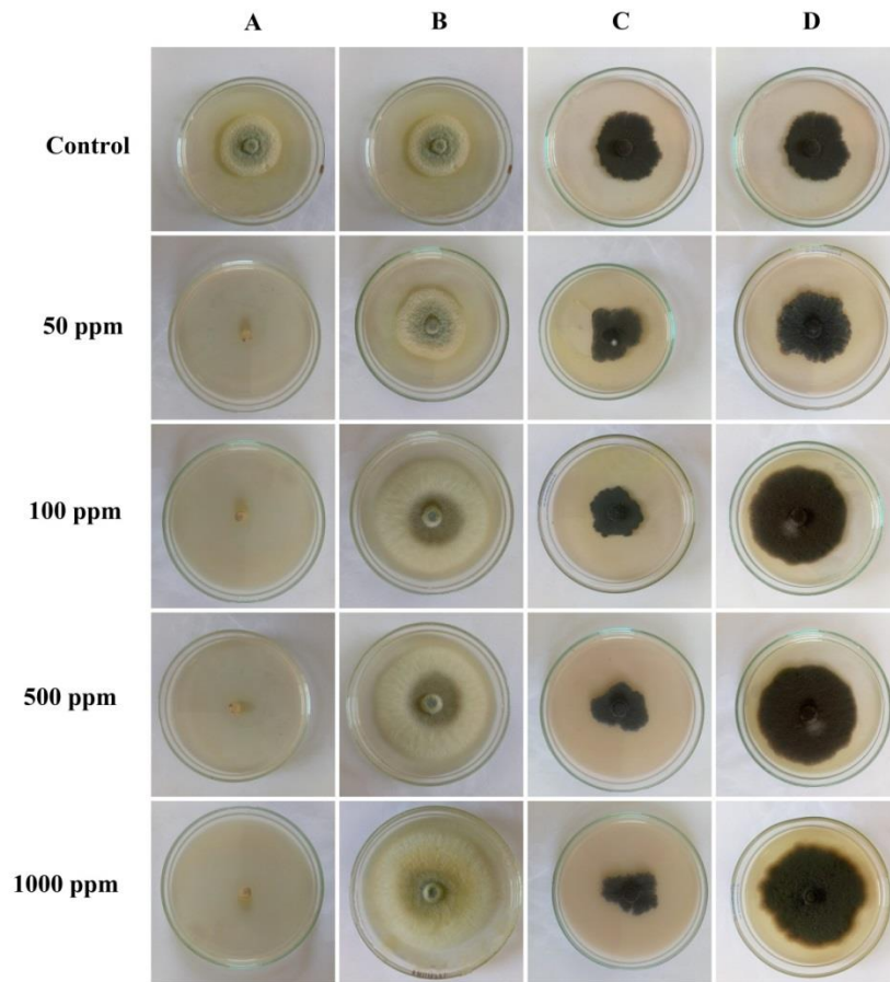
Fig. 3. Colony diameter of B. verrucosum and C. specifer on different concentration of fungicides, A: B. verrucosum on Scabdel, B: B. verrucosum on Golden Copper, C: C. specifer on Scabdel and D: C. specifer on Golden Copper.
